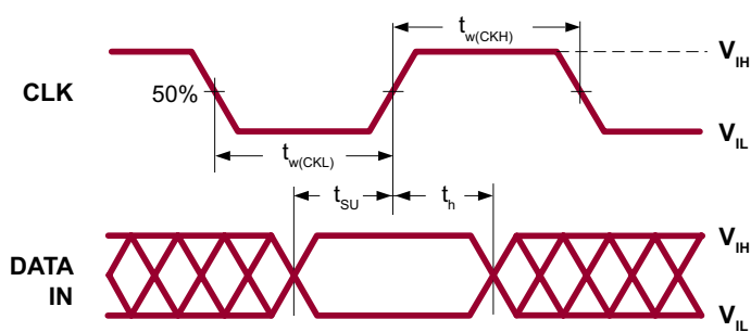
Figure 1: Input Timing Voltage Waveforms
